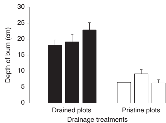
Figure 4 | Effects of experimental drainage on depth of ground fuel
