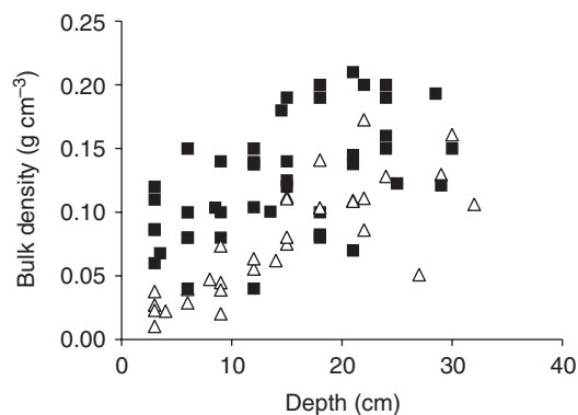
Figure 3 | Long-term drainage led to the formation of dense surface soils.
